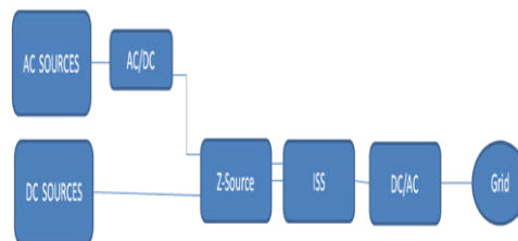
Fig 1 Dual Input Z Source Indirect Matrix Converter.
