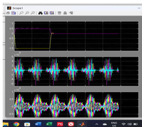
Fig 5 Dual Input Z Source Converter Final Output Wave From.
