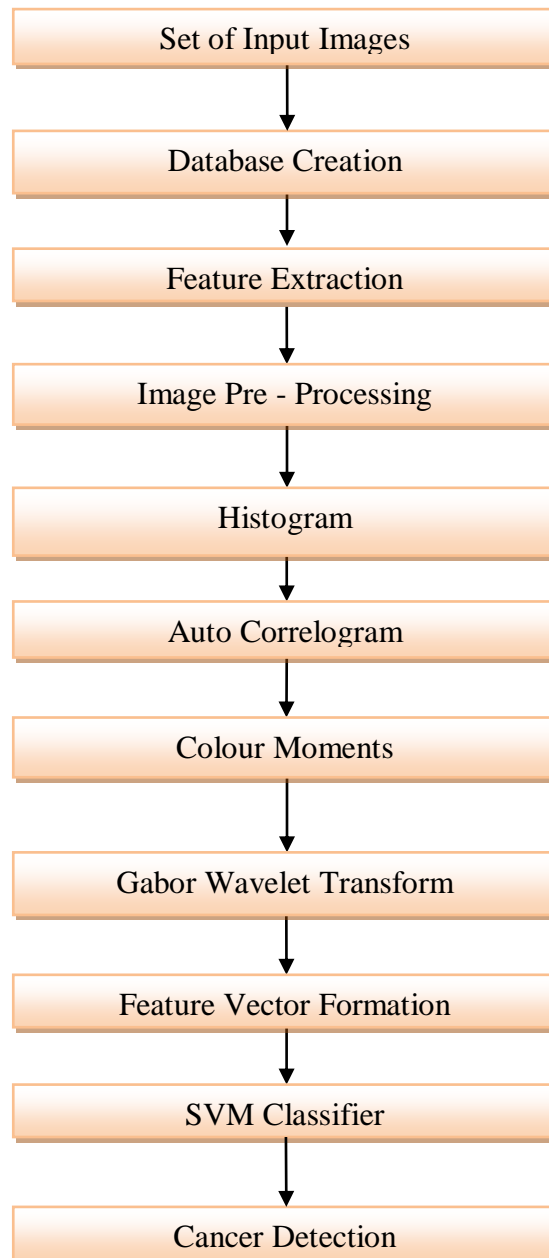
Figure 2 – The Flow of Skin Cancer Detection Using SVM
