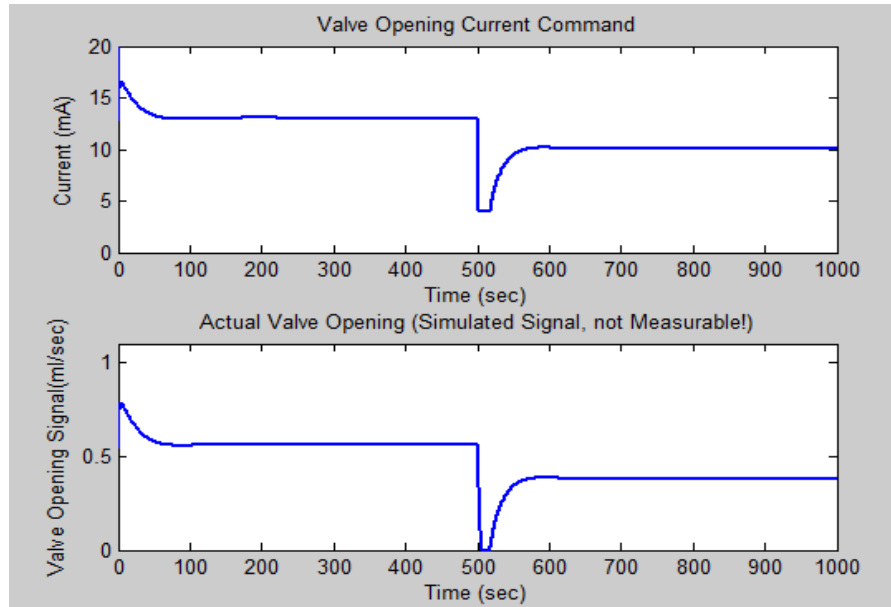
Fig. 4 Valve Opening Signals
