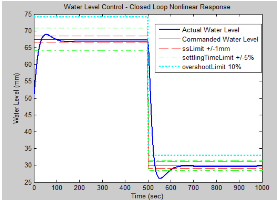
Fig. 3 Closed loop non linear response of the canal system
