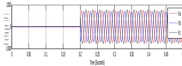
Fig. 9 Three phase Electric Spring voltage
