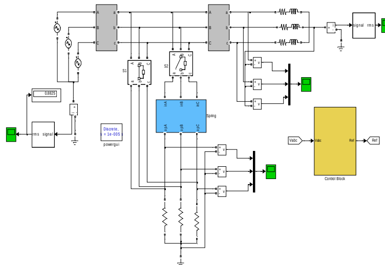
Fig. 4 Simulation Model for the Reduction of Neutral Current
