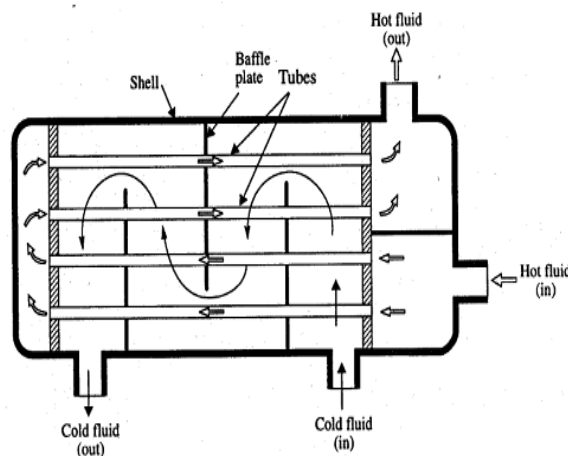
FIG: Shell and tube type heat exchanger
