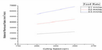
Figure 5.9 Depth of Cut as 1 mm
