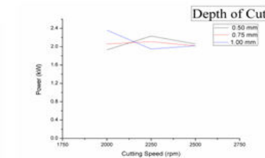
Figure 5.20 Feed Rate as 0.3 mm/rev
