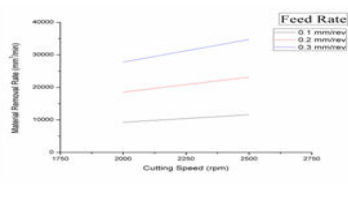
Figure 5.7 Depth of Cut as 0.5 mm
