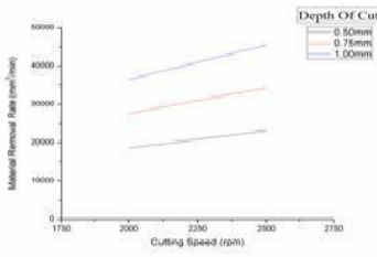
Figure 5.5 Feed Rate as 0.2 mm/rev
