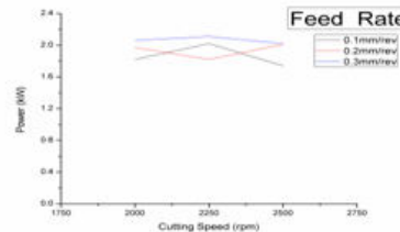
Figure 5.22 Depth of Cut as 0.75 mm
