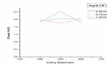
Figure 5.19 Feed Rate as 0.2 mm/rev
