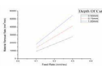
Figure 5.1 Cutting Speed as 2000 rpm
