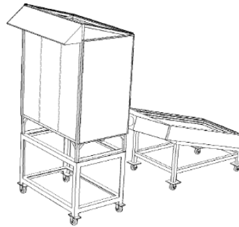
Fig 2. The schematic diagram of the dryer
