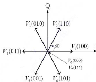
Fig.3 Eight possible voltage space vectors
