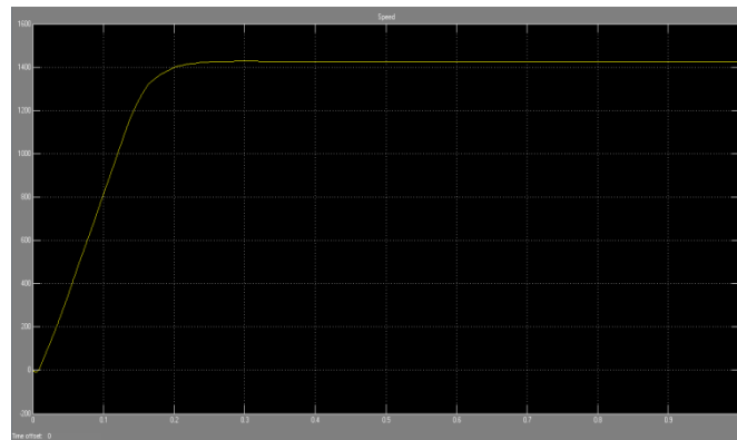
4.14 Fig : Speed in DTC
