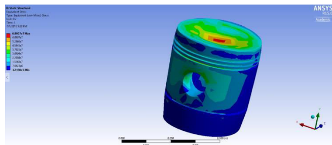
Fig. 2: outline plot of corresponding (Von-mises) tension in piston
