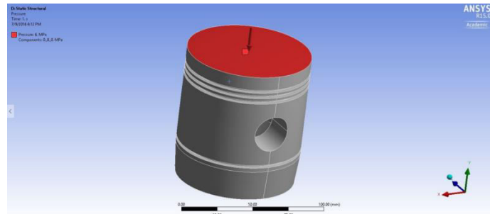
Fig. 1: Applied pressure with fixed support
